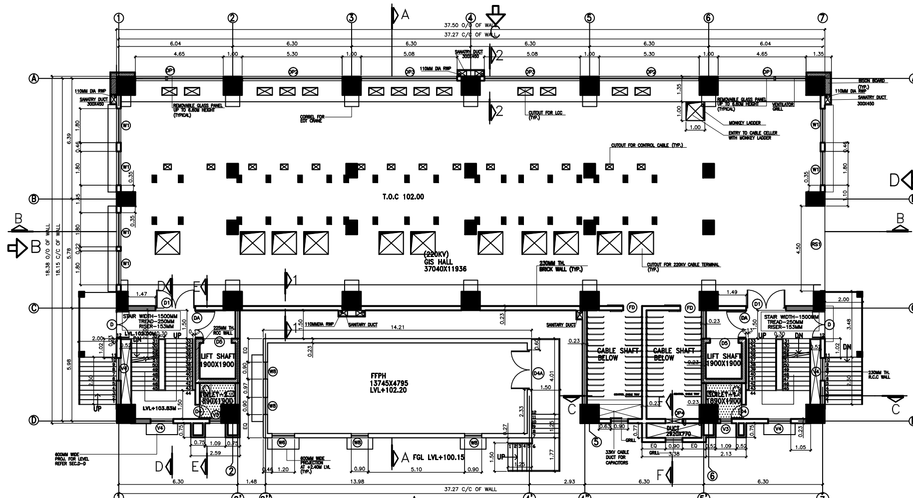
GROUND FLOOR PLAN ( T.O.C 102.00LVL)
