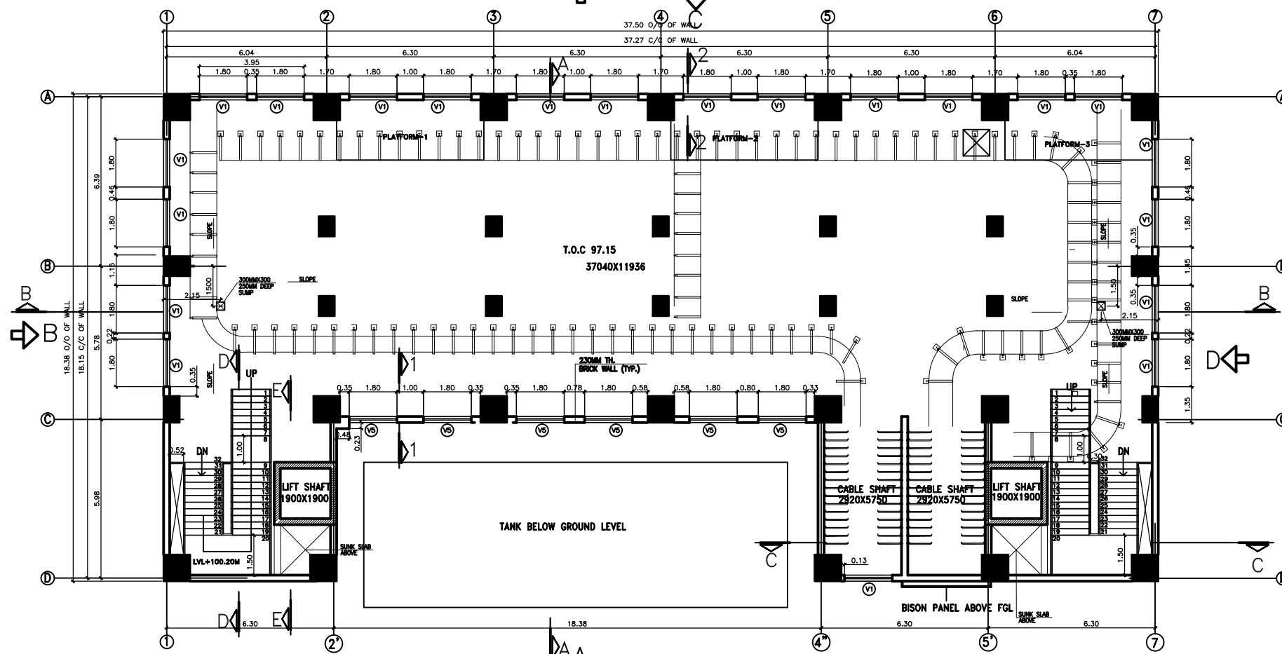
BASEMENT FLOOR PLAN (T.O.C 97.15 TO 97.7)
